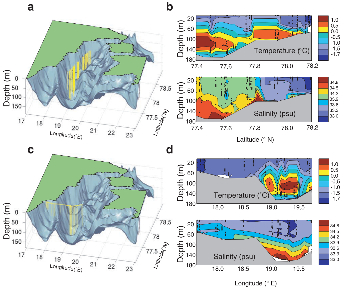
Figure 3. CTD transects in Storffjorden, Svalbard. The maps show the locations of selected dives performed by a white whale (each yellow spike represents a dive; the length of the spikes represents dive depth) carrying a CTD tag, along a north-south transect (a) and an east-west (c) transect superimposed on a three-dimensional bathymetric map of Storffjorden, Svalbard. CTD-casts produced during these dives are the basis for the temperature and salinity profiles shown in b and d respectively. Each dot in b and d represents a location where a CTD-measurement was taken.
